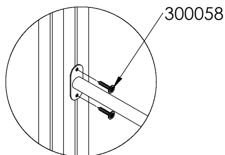
DETAIL R SCALE 1 : 10
