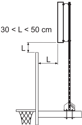
Side view on basketball backboard
