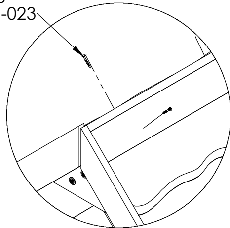
DETAIL T SCALE 1 : 10
