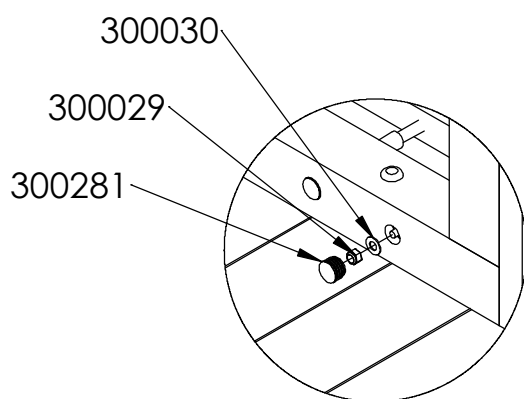
DETAIL P SCALE 1 : 10
