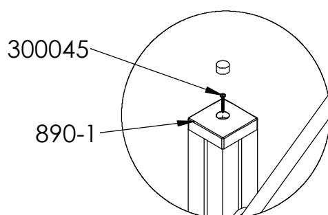
DETAIL AC SCALE 1 : 10
