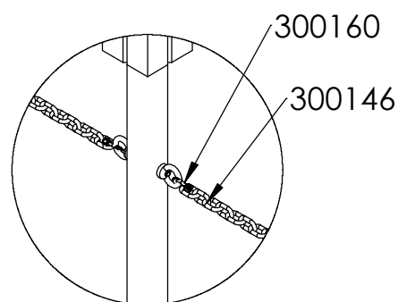
DETAIL V SCALE 1 : 10
