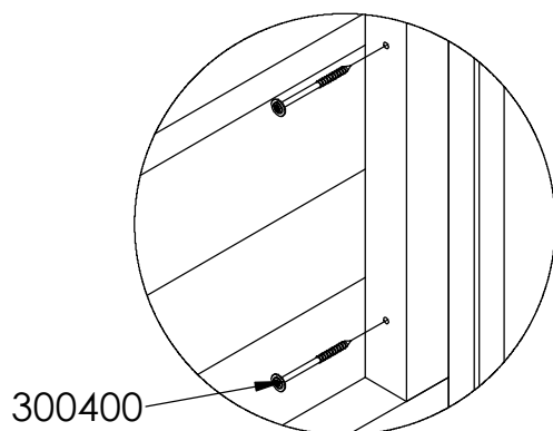
DETAIL R SCALE 1 : 10
