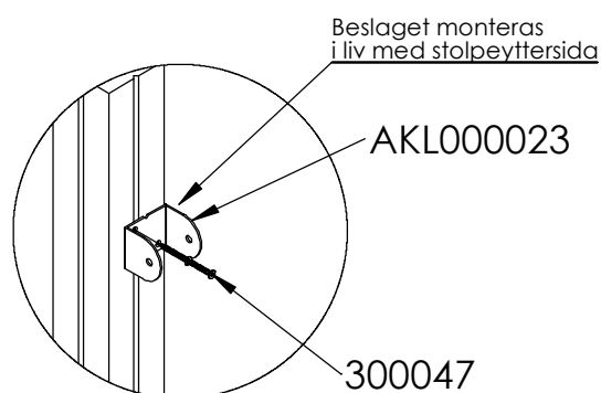
DETAIL C SCALE 1 : 10
