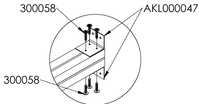
DETAIL P SCALE 1 : 10
