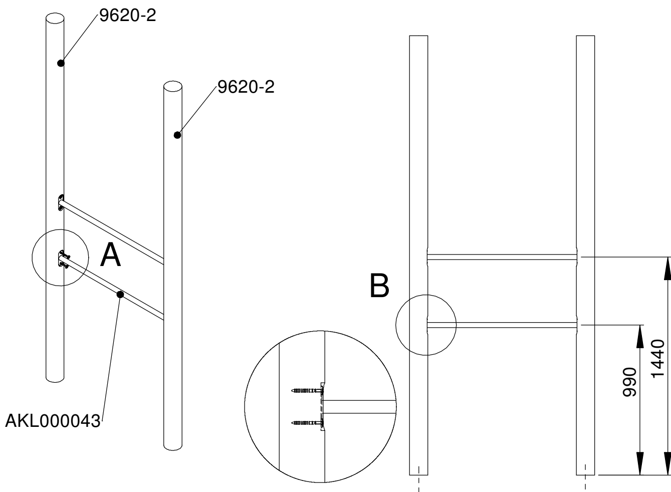
300059 DETAIL B SCALE 1 : 10
