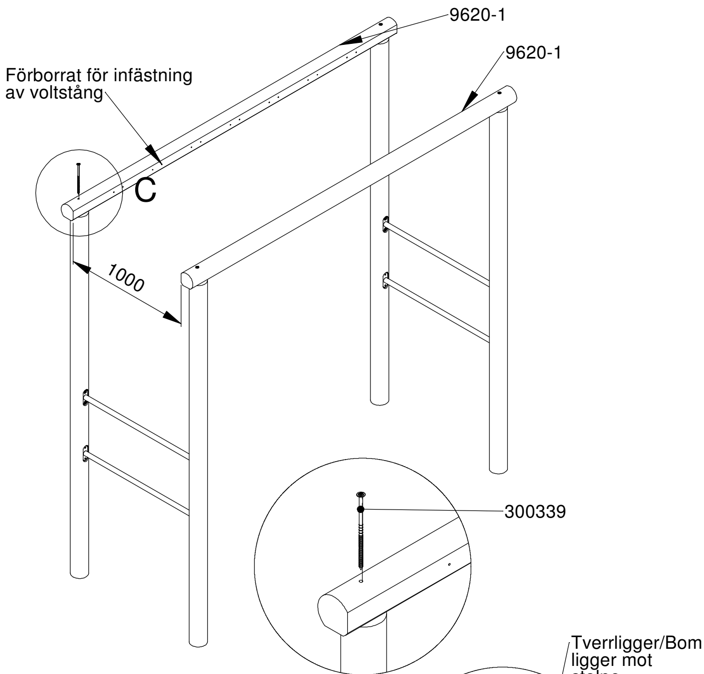
DETAIL C SCALE 1 : 10
