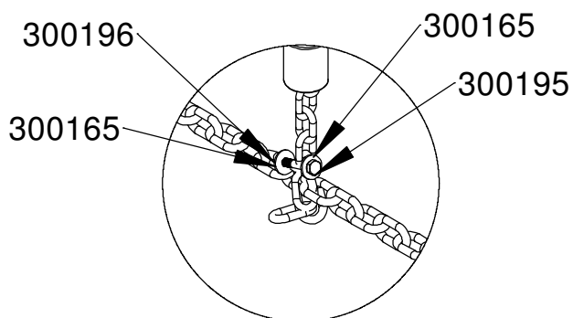
DETAIL D SCALE 1 : 5
