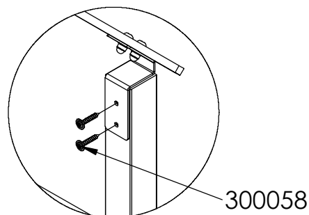
DETAIL Q SCALE 1 : 10
