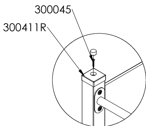
DETAIL M SCALE 1 : 10
