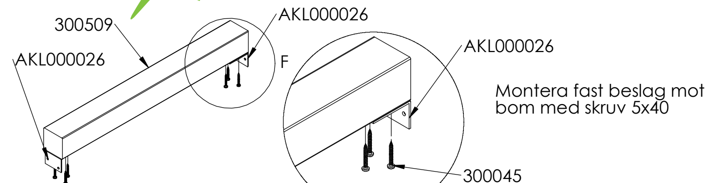
DETAIL F SCALE 1 : 5
